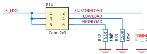
Figure 17: Load switch and LDO schematic
