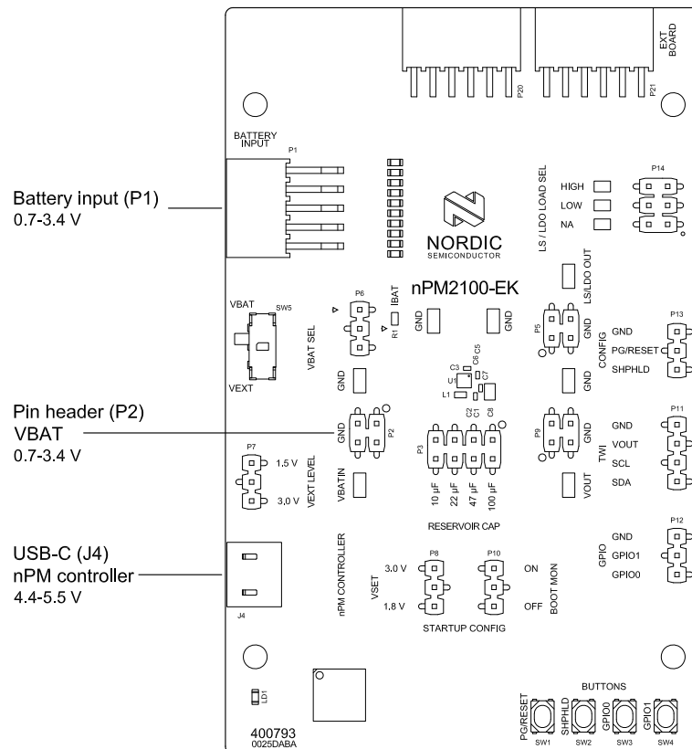
Figure 6: Power supply
