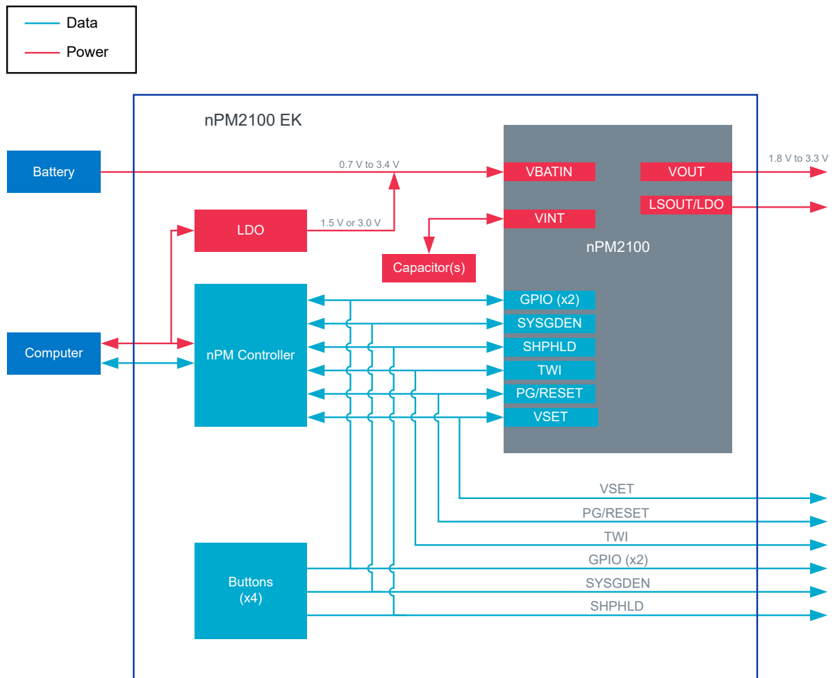
Figure 5: Block diagram
