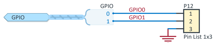
Figure 10: GPIO schematic
