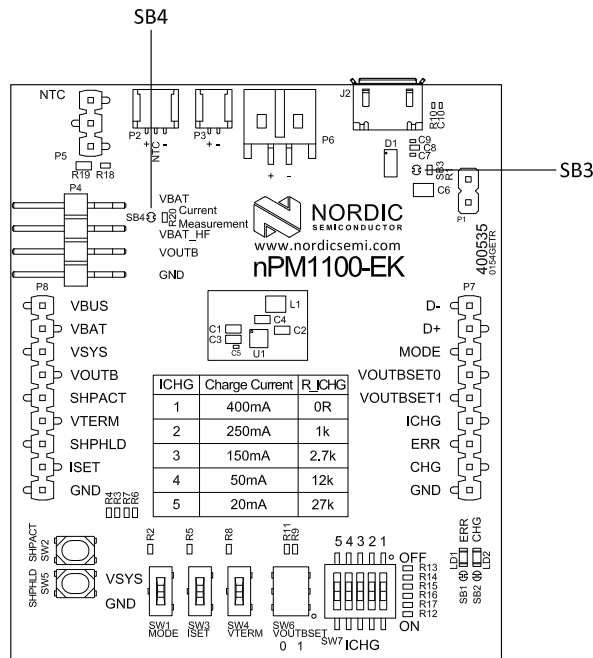
Figure 8: Prepare the EK for current measurements
