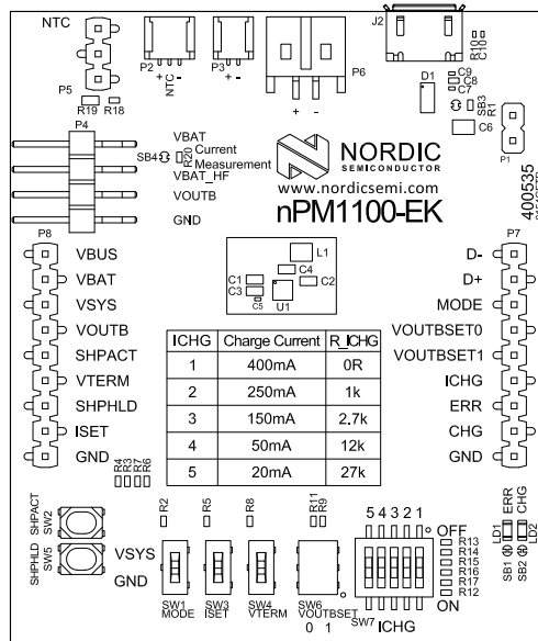
Figure 3: nPM1100 EK front view
