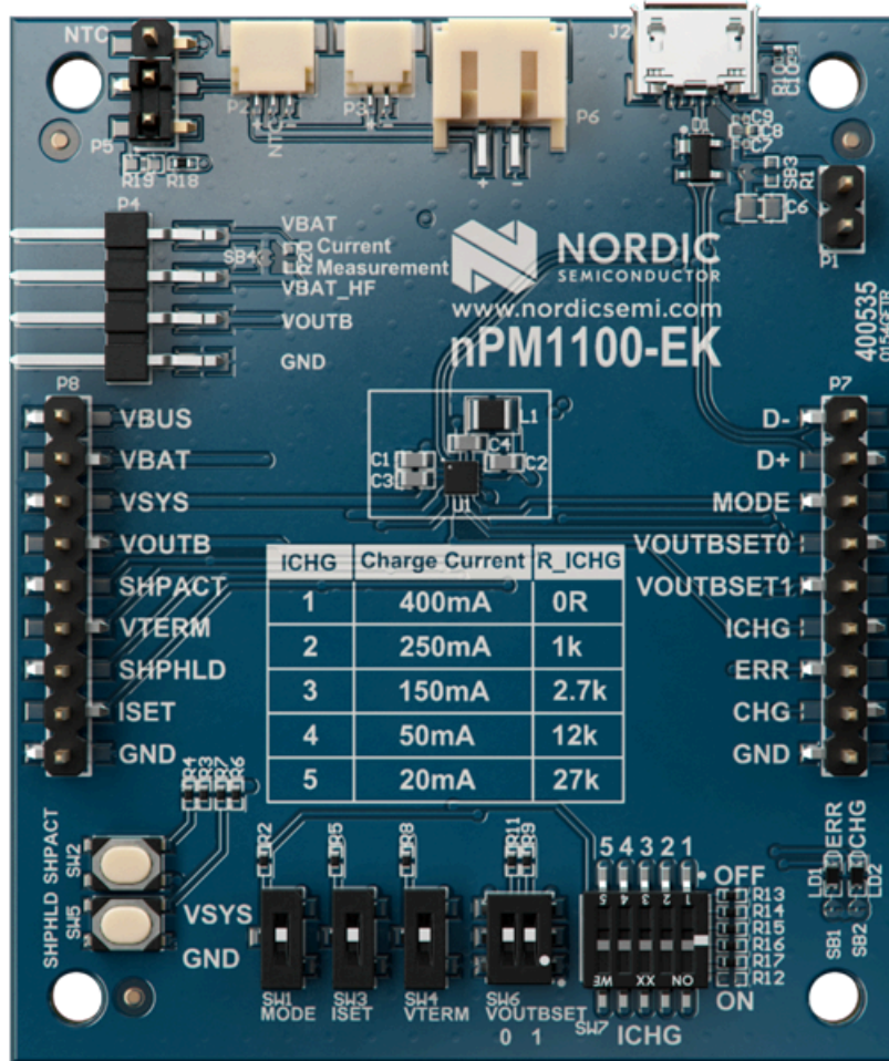
Figure 1: nPM1100 EK (standard)
