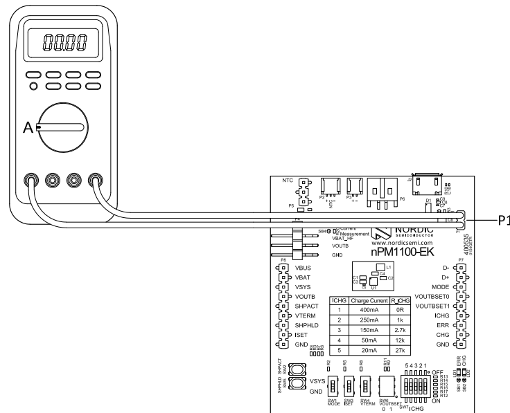
Figure 10: VBUS current measurement with an ampere meter
