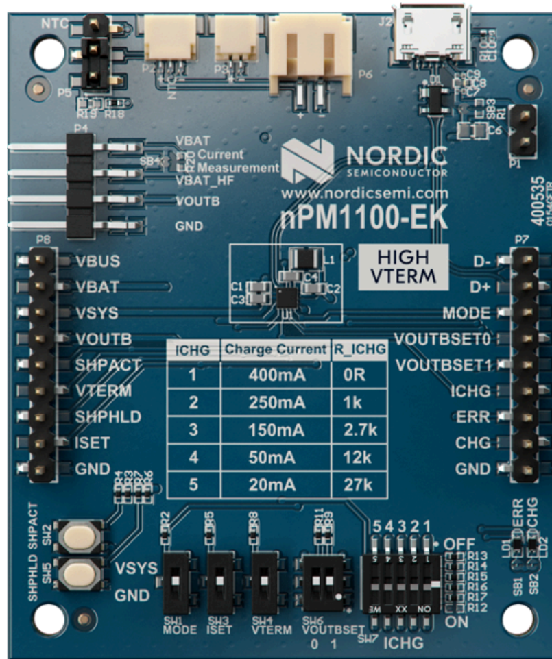
Figure 2: nPM1100 EK (HIGH VTERM)
