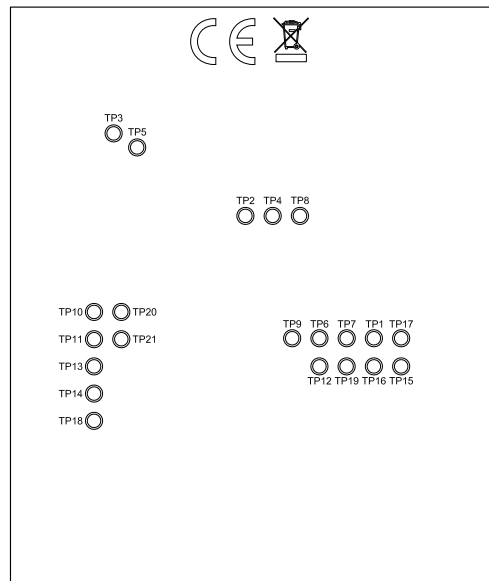
Figure 4: nPM1100 EK back view
