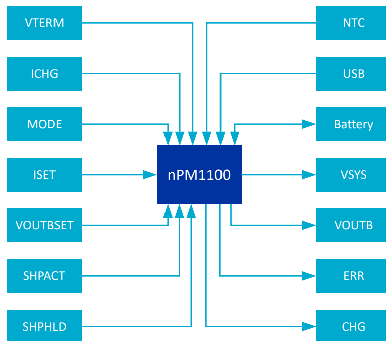
Figure 5: nPM1100 EK block diagram
