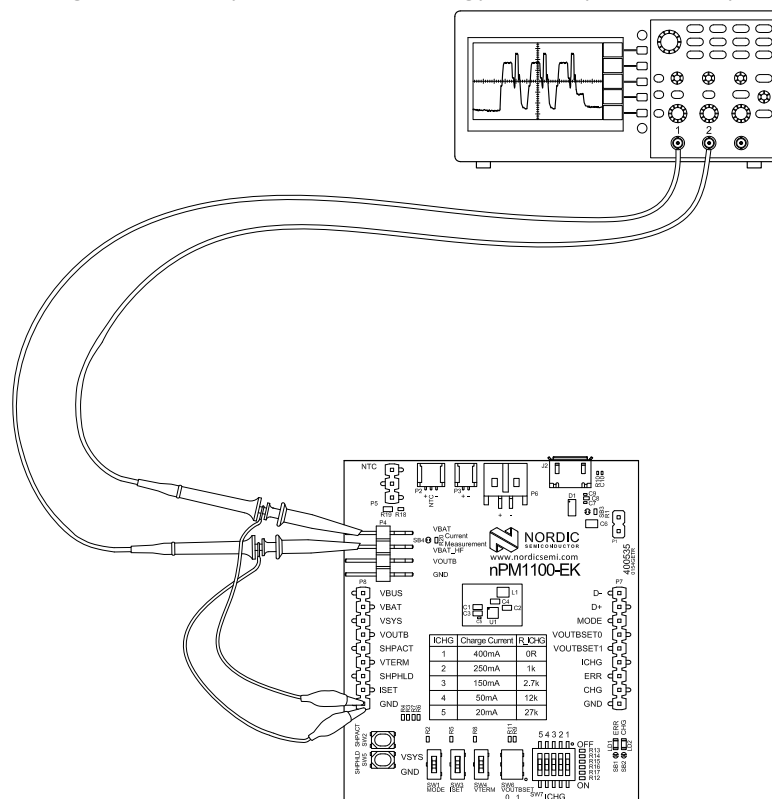
Figure 9: VBAT current measurement with an oscilloscope
